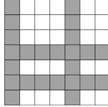
Figure 1: The multi-grid construction, n = 7 \times 7 , b = 3 , with one quorum shaded.
