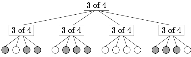
Figure 2: An \text{RT}(4, 3) system of depth h = 2 , with one quorum shaded.
