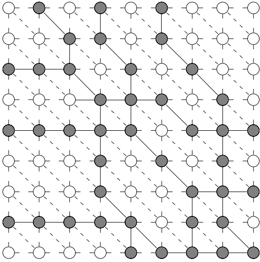
Figure 3: A multi-path construction on a 9 \times 9 grid, b = 4 , with one quorum shaded.
